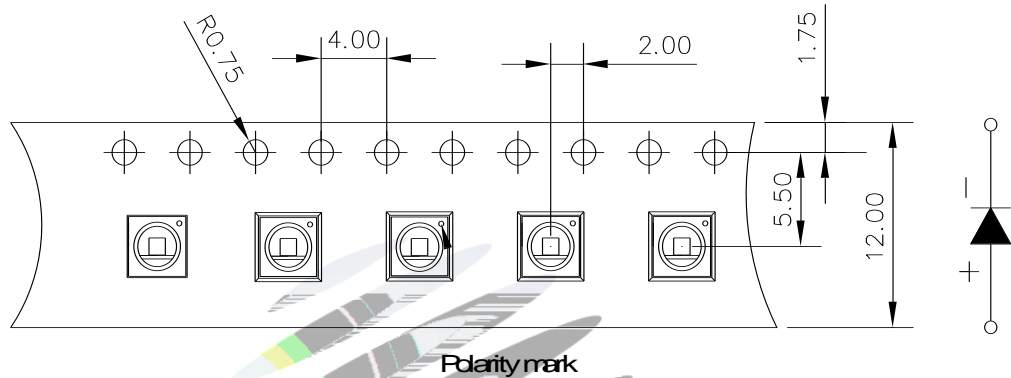
Fig.2-1 Carrier Tape Dimension 载带尺寸
