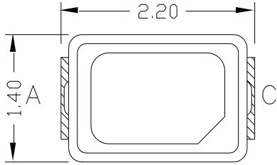
Fig. 1-1 Top view
