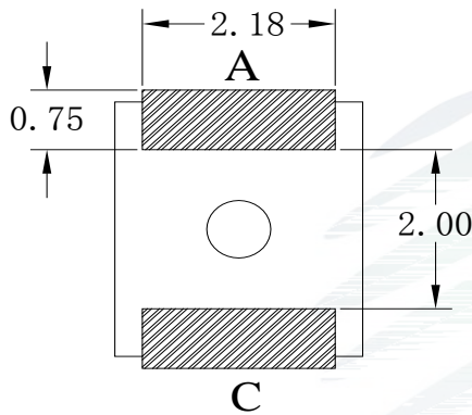
Fig. 1-1 Top View
