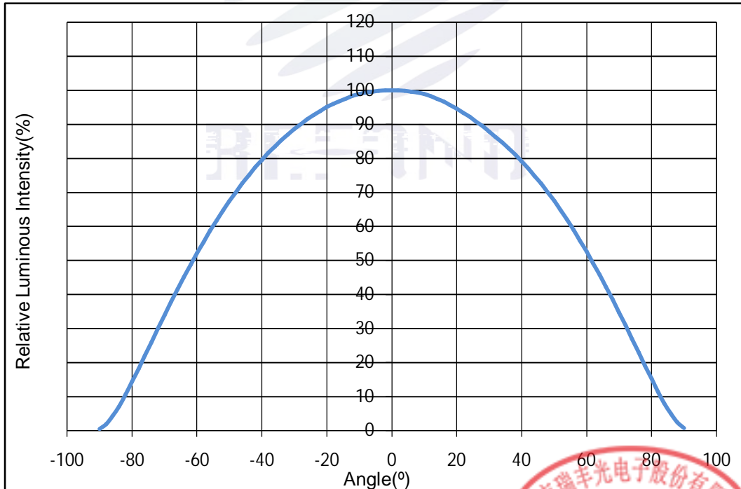
Fig. 1-12 Radiation diagram
