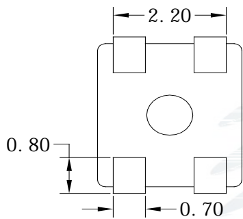
Fig. 1-3 Bottom View
