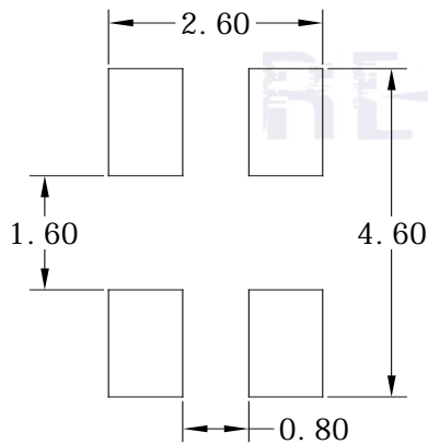
Fig. 1-5 Soldering Patterns
