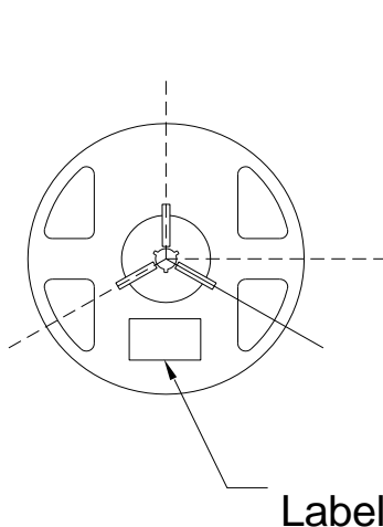
Fig.2-2 Reel 卷盘
