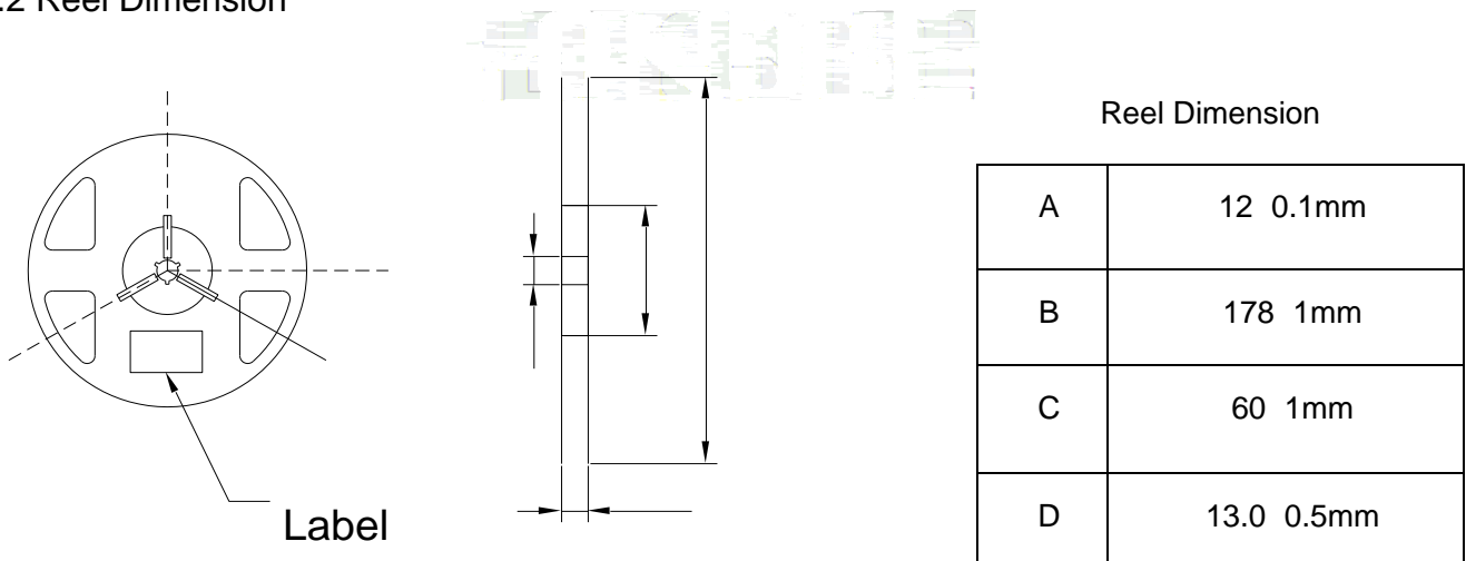
Fig.2-2 Reel Dimension
