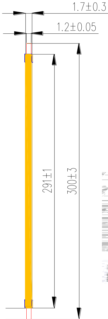
Fig.1-1 Top view
