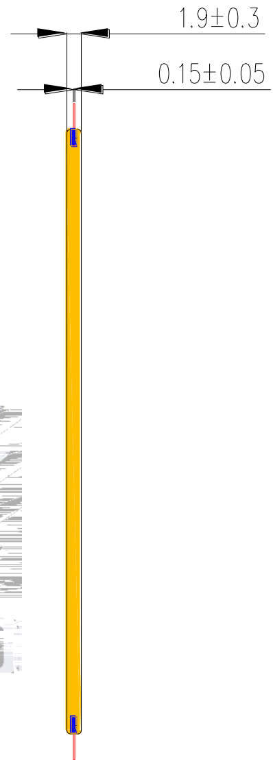
Fig.1-2 Bottom view
